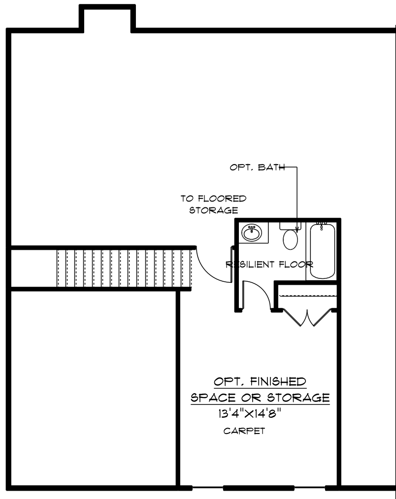
OPTIONAL SECOND FLOOR PLAN - 308 S.F.(FIN.)
